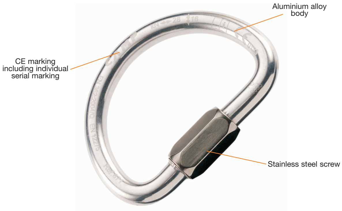
Connection to the "A/2" attachment points of a fullbody harness and to a lanyard
